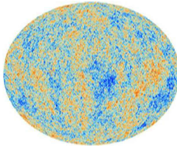
Figure 1. cosmic microwave according to the Planck the Planck Collaboration
